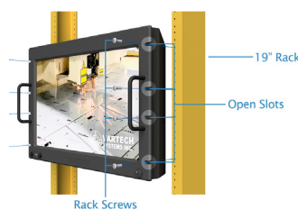
Rack
