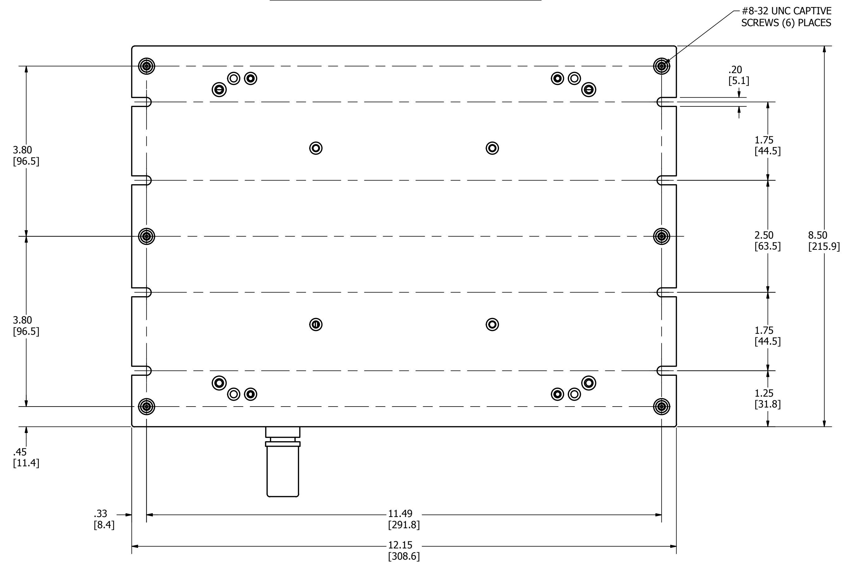
POWER CUBE 2 WITH RIGID MOUNT
