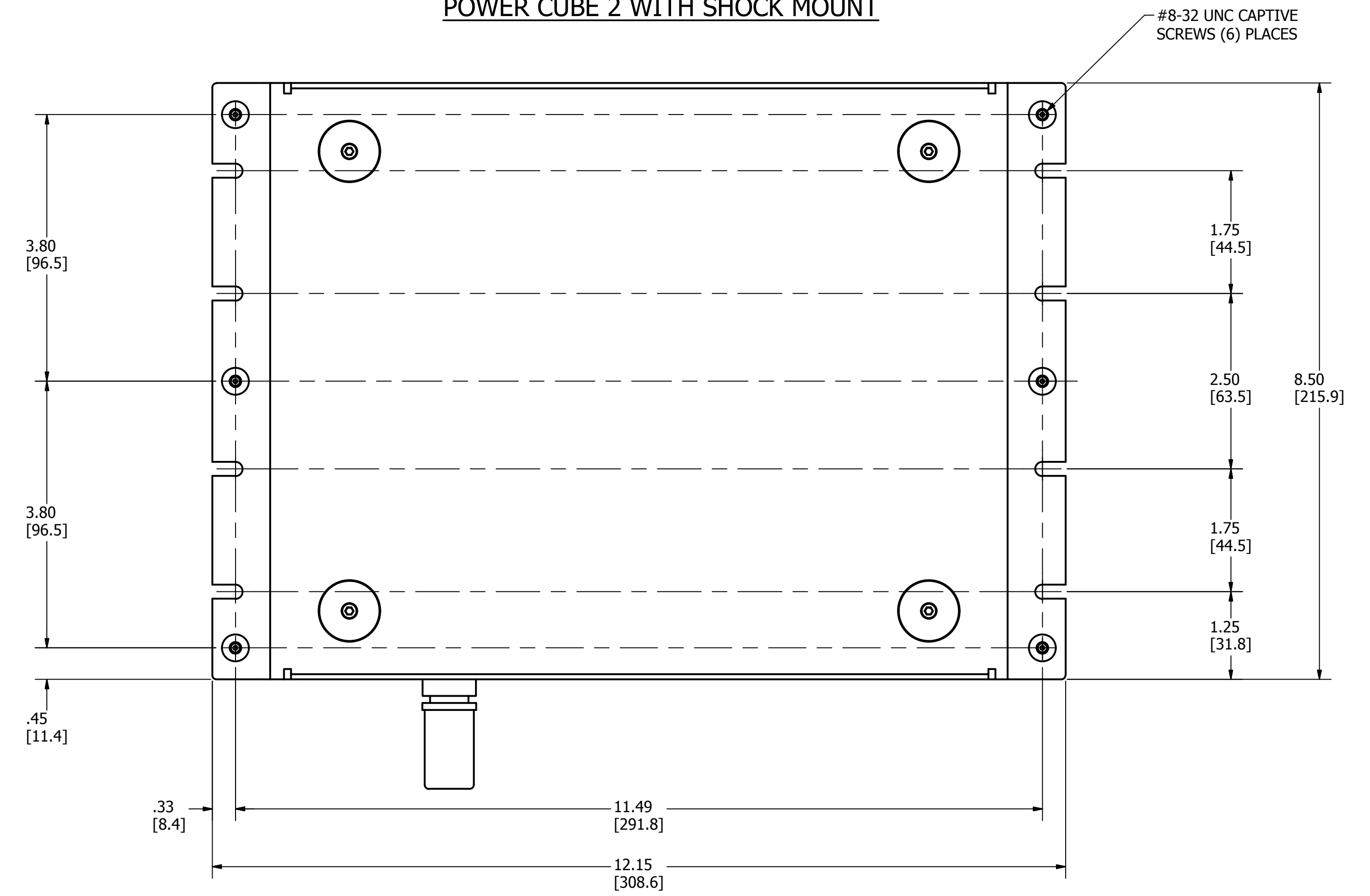
POWER CUBE 2 WITH SHOCK MOUNT
